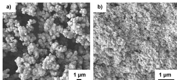
Figure 1. SEM images of PICU synthesized in DMF at a) 80^\circ\text{C} and b) 25^\circ\text{C} .
