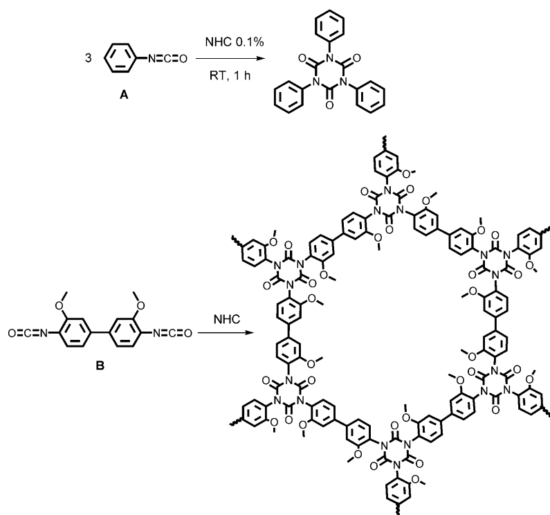
Scheme 1. Synthesis of PICU.
