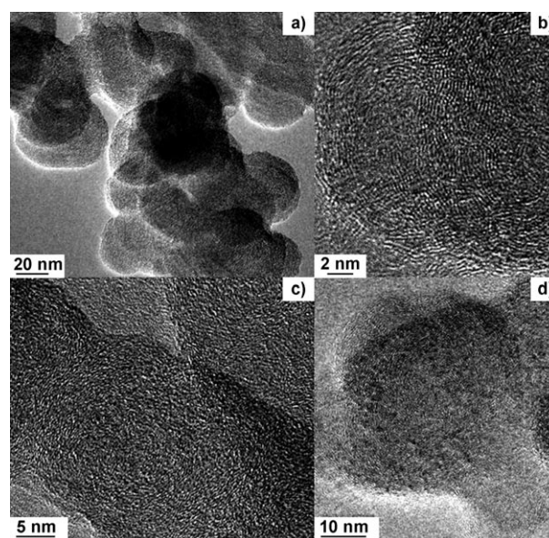
Figure 3. TEM images of Fe/PICU a,b) before reaction, c) after the first run, and d) after the fifth run.
