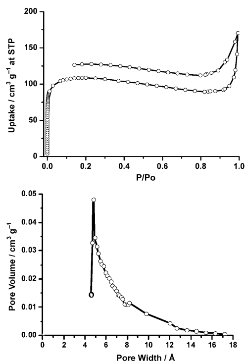
Figure 2. Nitrogen adsorption-desorption isotherm and pore size distribution of PICU.
